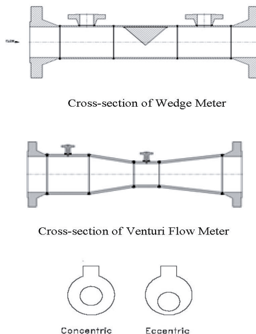
Concentric and Eccentric Orifice Plates, Viewed Parallel to Flow Figure 5. Types of Flow Meters for Wet Gases.
