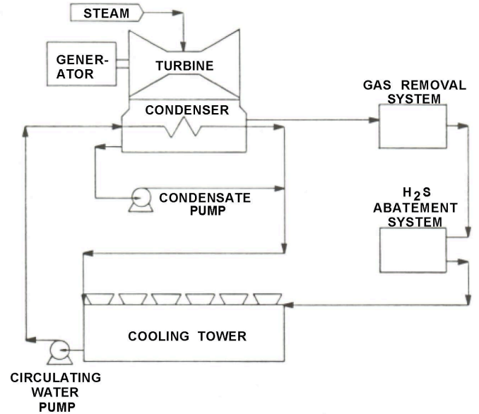
Source: "The Geysers Unit 1, Pacific Gas and Electric Company," National Historic Mechanical Engineering Landmark, The American Society of Mechanical Engineers, October 1985, p. 7. (Although the source for Figure 1 mentions Unit 1, Figure 1 does not depict Unit 1 but rather later units.)
